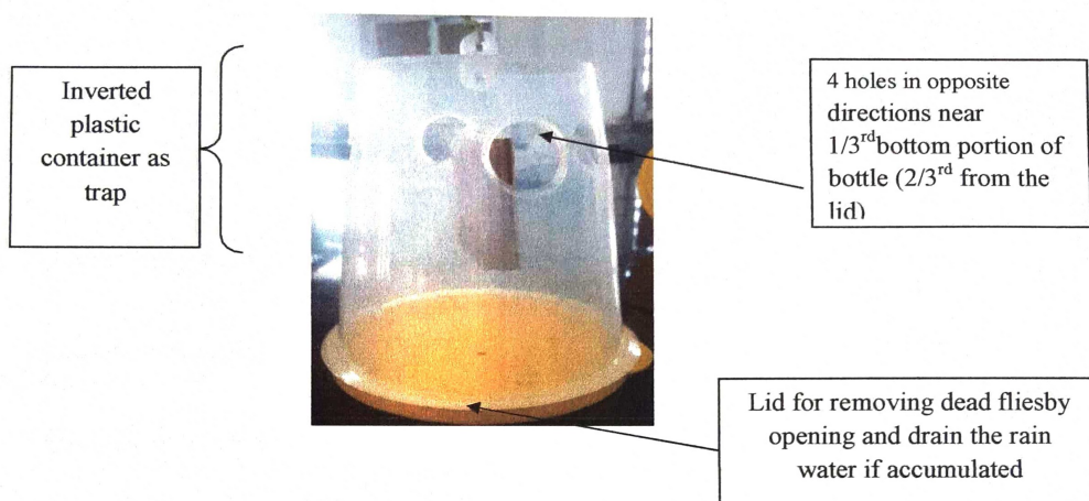
Fig.-3 Trap assembly with killing block
